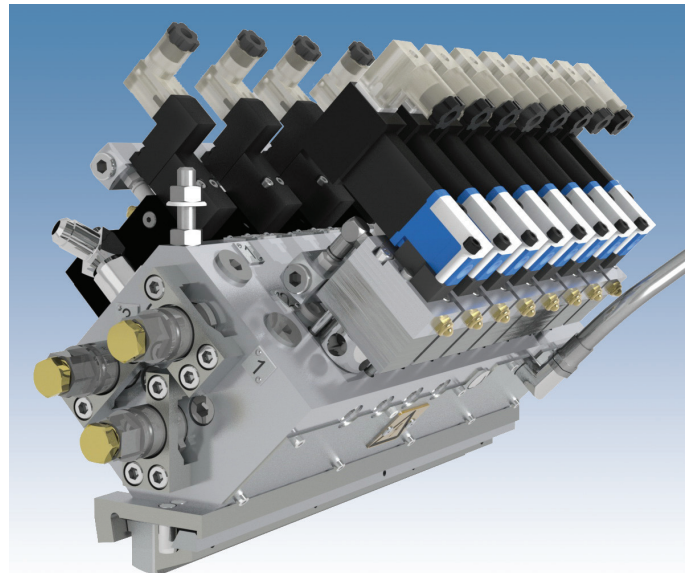
Trio slot applicator with quick-exchange nozzle & adapter
